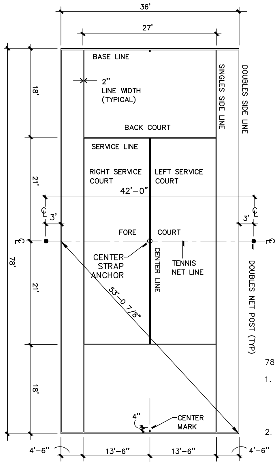
78 FOOT TENNIS COURT PLAYING LINE LAYOUT
