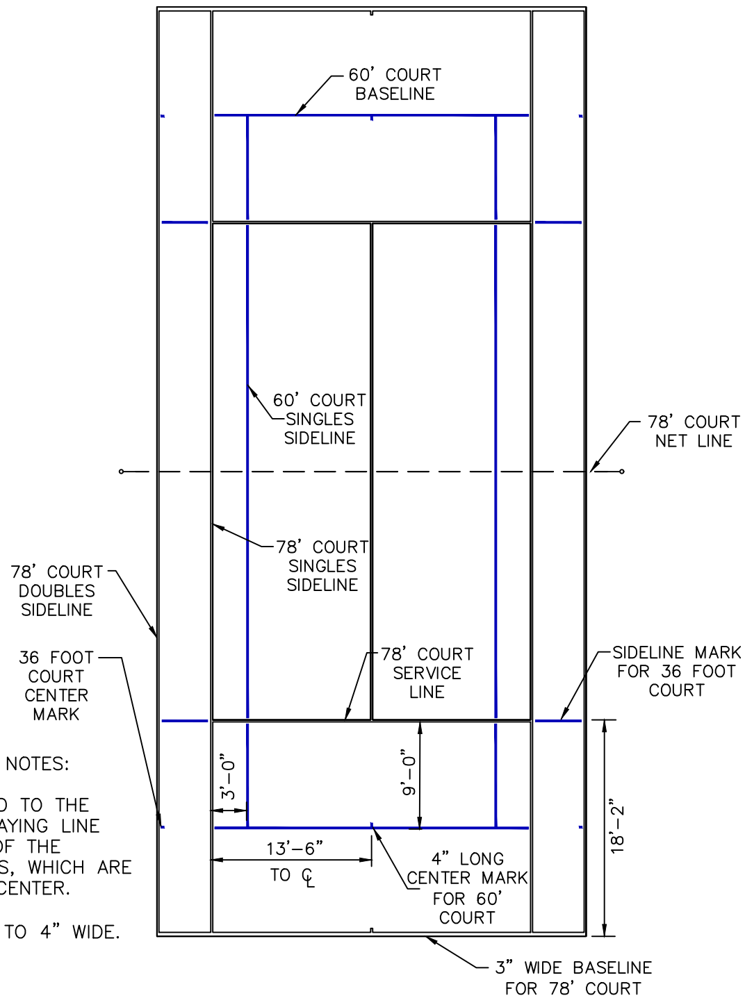
36/60 FOOT TENNIS COURT PLAYING LINE LAYOUT
