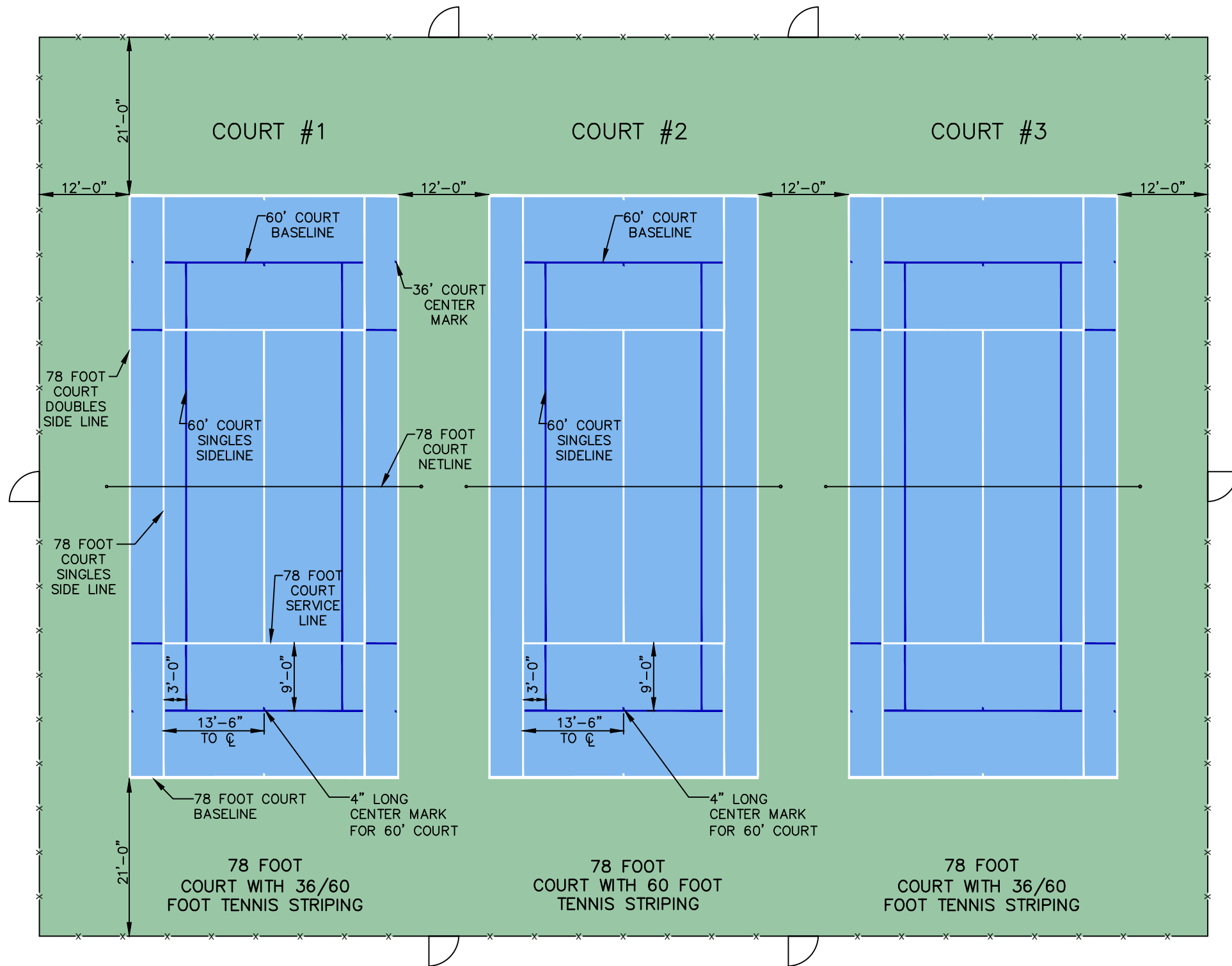
THREE 78 FOOT TENNIS COURTS WITH BLENDED PLAYING LINES NOT TO SCALE
