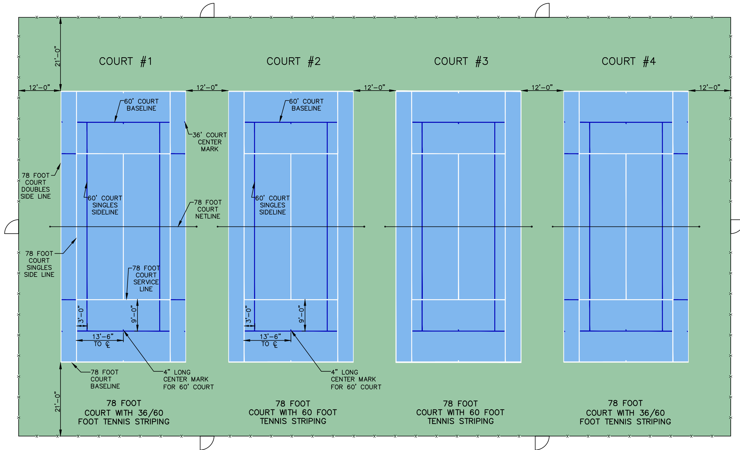
FOUR 78 FOOT TENNIS COURTS WITH BLENDED PLAYING LINES NOT TO SCALE
